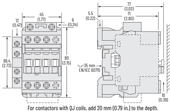
Figure 40 - 100-E09...100-E16 Contactors with Low-consumption Coils and Side-mounted Auxiliary Contact
